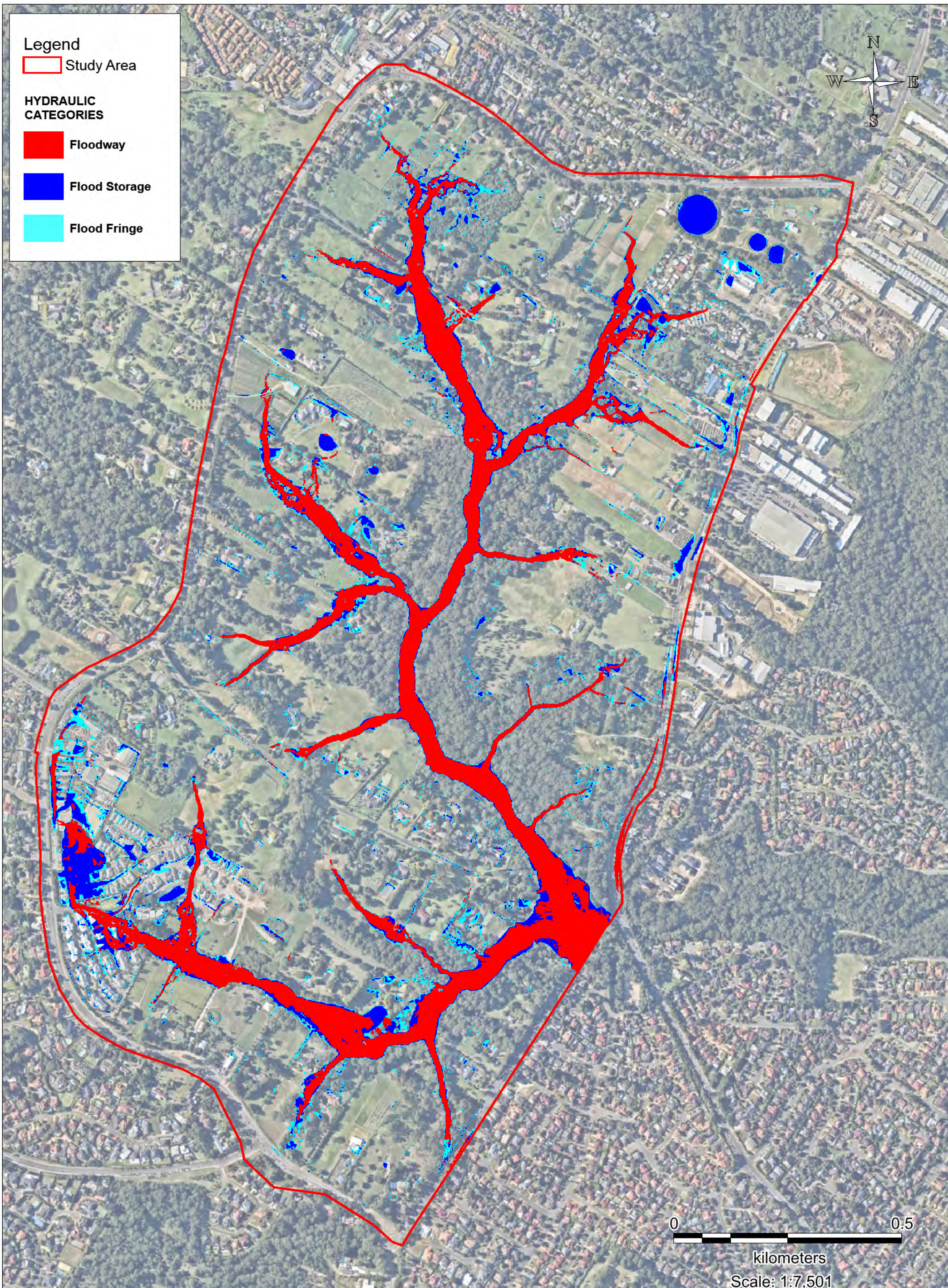
Figure B16 - PMF Hydraulic Categories - Existing Conditions
