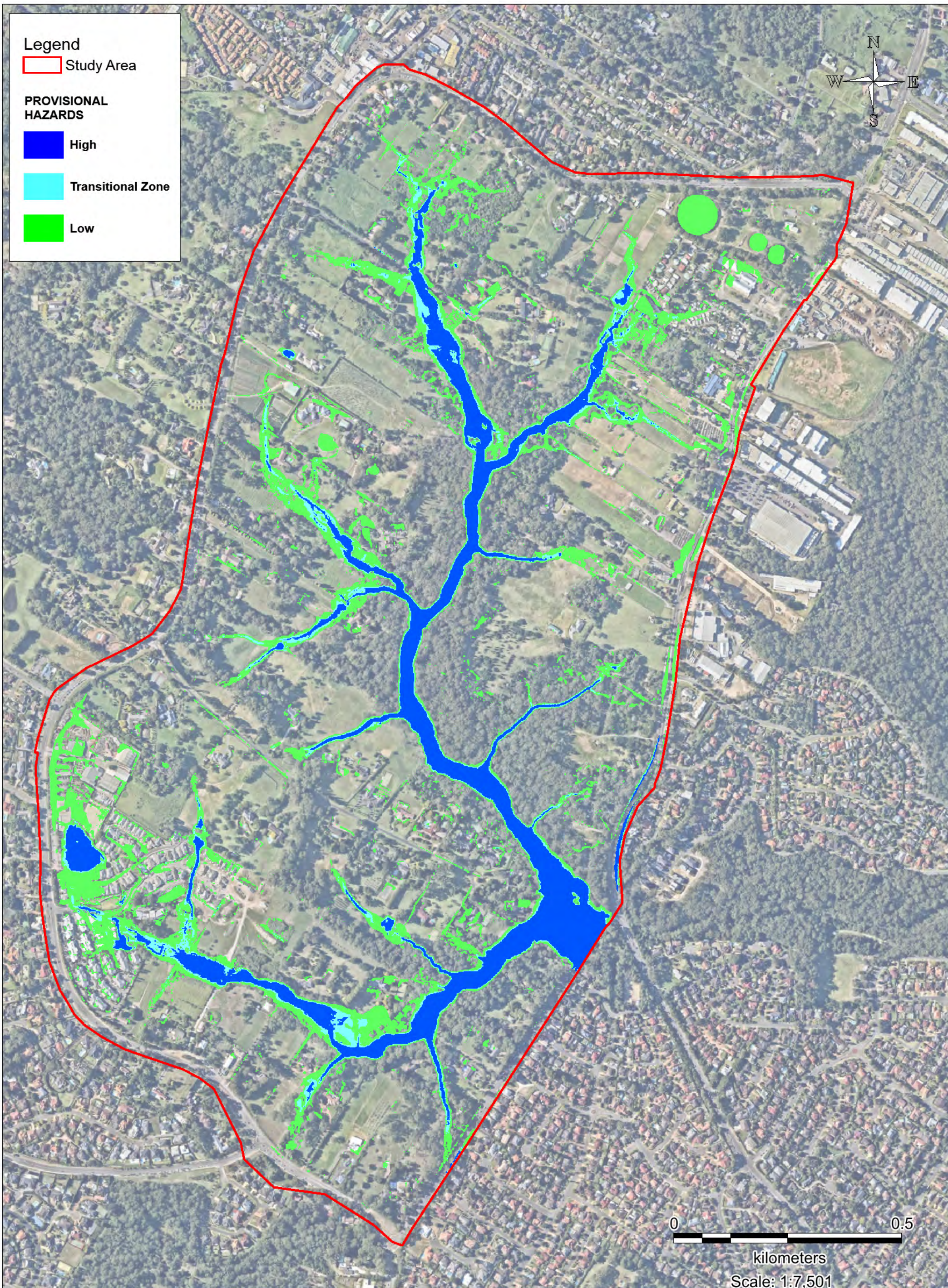
Figure B14 - PMF Provisional Hazards - Existing Conditions
